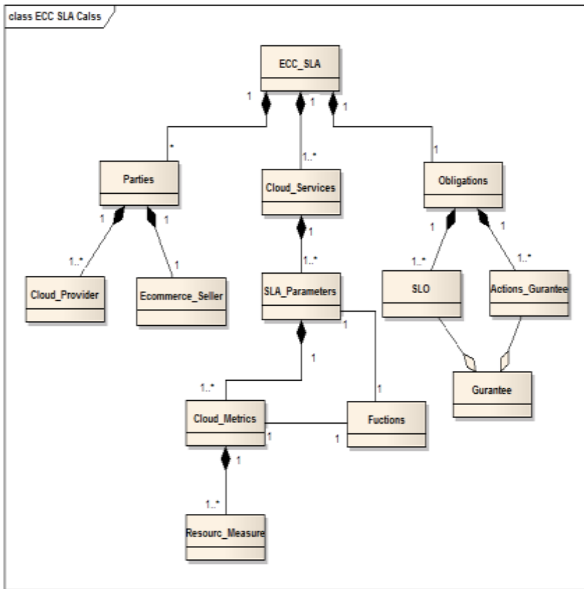
Figure 3. Ecommerce cloud SLA Document Structure.
