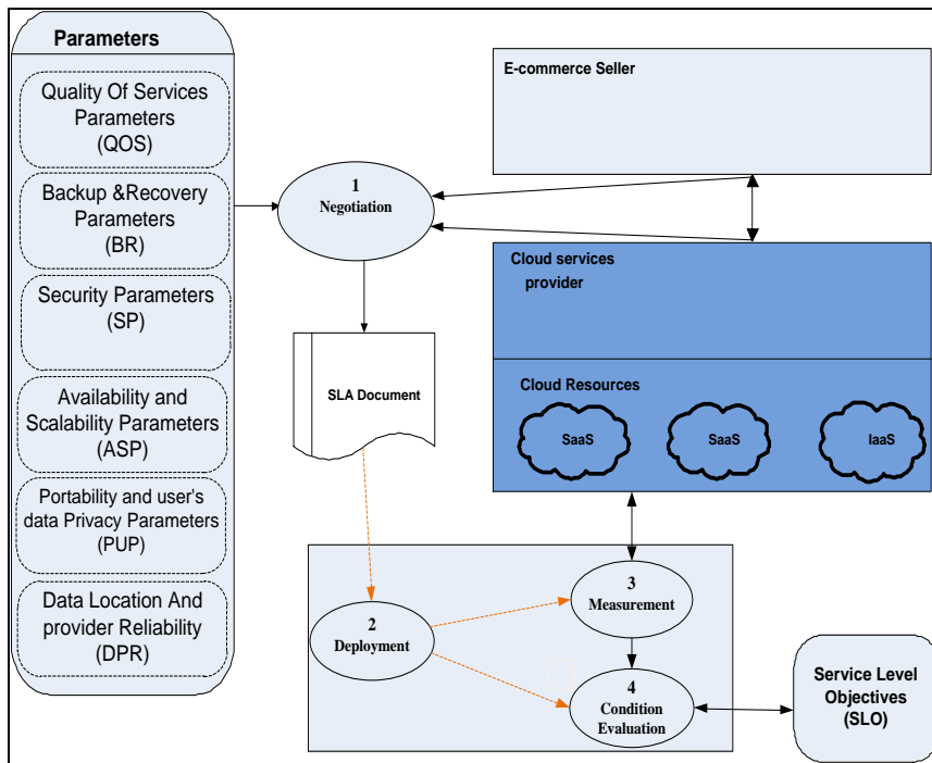
Figure 2. Ecommerce Cloud Service Level Agreement Framework.
