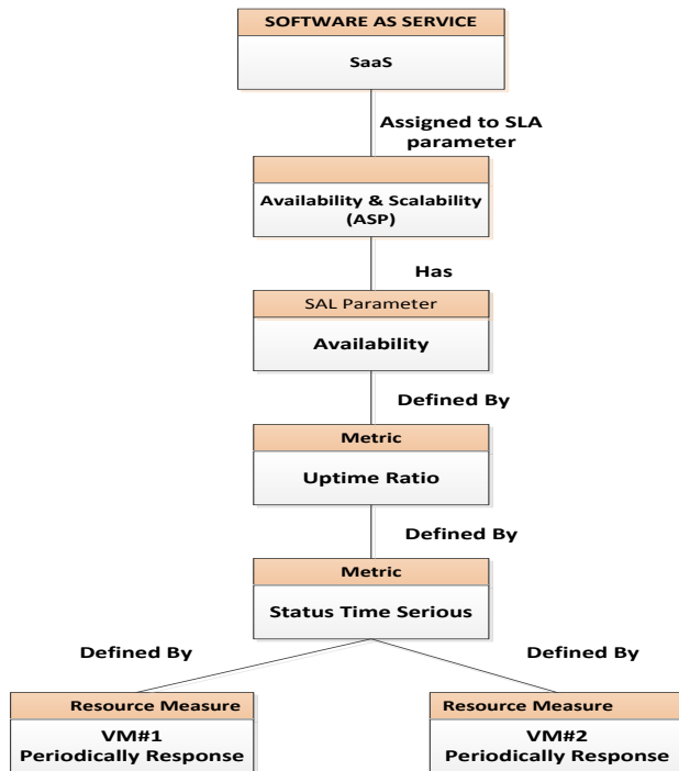
Figure 4. Structure of defining Availability parameters.
