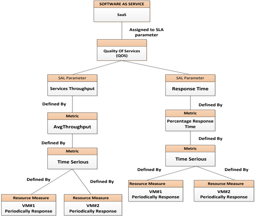
Figure 5. Structure of defining quality of services parameters.
